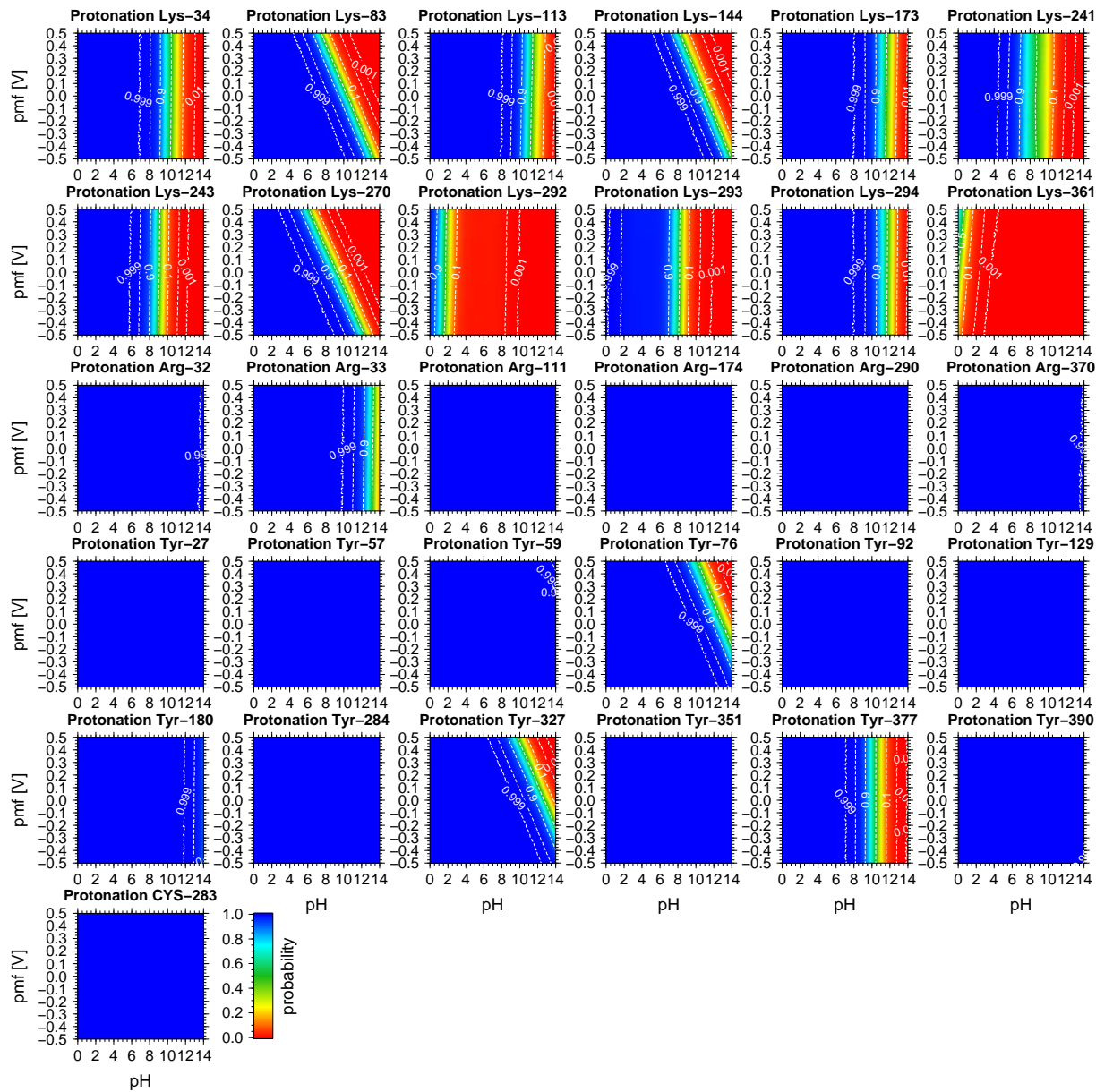
Figure S14: Titration curves pH - \Delta\psi II. Continued from Fig. S13. See caption of Fig. S13 for explanation.
