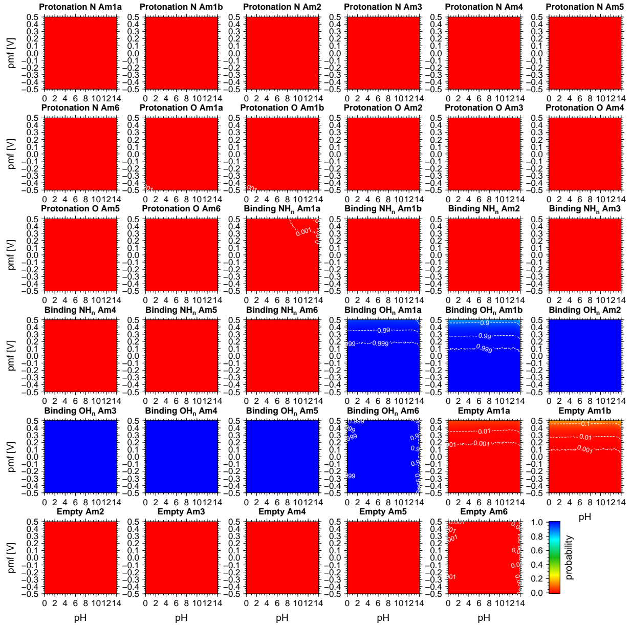
Figure S15: Titration curves \text{pH} - \Delta\text{pH} + \Delta\psi III. Probability for binding states of the sites in the transmembrane pore as a function of the intracellular pH value and a pmf consisting of a transmembrane pH difference and an electric transmembrane potential. The ratio of the pH difference to the electric transmembrane potential is given by \frac{\Delta\psi}{\Delta\text{pH}} = 2 . The sites and the specific binding probabilities are indicated by the labels above the curves. Protonation N indicates the conditional probability of binding an ammonium ion under the condition that either ammonium or ammonium is bound to the site. Protonation N indicates the conditional probability of binding an hydronium ion under the condition that either water or an hydronium ion is bound to the site. Binding \text{NH}_n indicates the probability of binding ammonia or an ammonium ion to the site. Binding \text{OH}_n indicates the probability of binding any water species (water, hydronium ion or hydroxide ion) to the site.
