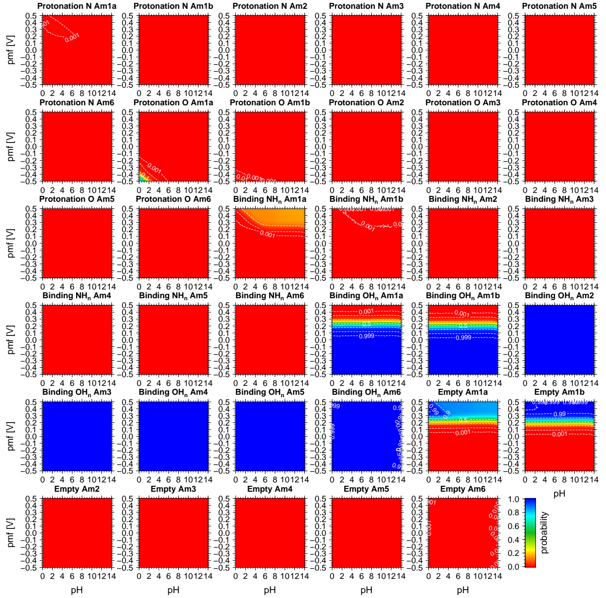
Figure S7: Titration curves \text{pH} - \Delta\text{pH} III. Probability for binding states of the sites in the transmembrane pore, as a function of the intracellular pH value and a pmf consisting entirely of a transmembrane pH difference. The sites and the specific binding probabilities are indicated by the labels above the curves. Protonation N indicates the conditional probability of binding an ammonium ion under the condition that either ammonium or ammonium is bound to the site. Protonation N indicates the conditional probability of binding an hydronium ion under the condition that either water or an hydronium ion is bound to the site. Binding NH n indicates the probability of binding ammonia or an ammonium ion to the site. Binding OH n indicates the probability of binding any water species (water, hydronium ion or hydroxide ion) to the site.
