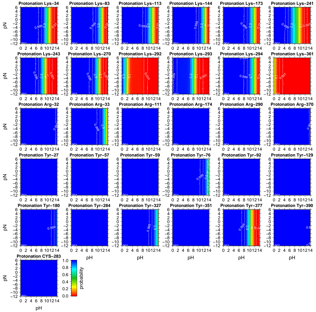
Figure S22: Titration curves intracellular pH - pN with pmf II., (pN equal on both membrane sides, \Delta\text{pH}=1.0 , \Delta\psi = -120 mV). Continued from Fig. S21. See caption of Fig. S21 for explanation.
