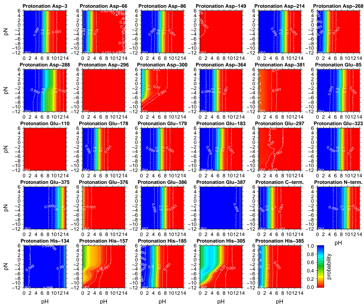
Figure S21: Titration curves intracellular pH - pN with pmf I. (pN equal on both membrane sides, \Delta\text{pH}=1.0 , \Delta\psi = -120 mV). Protonation probability as a function of the intracellular pH value and a pmf consisting of a transmembrane pH difference and an electric transmembrane potential. The ratio of the pH difference to the electric transmembrane potential is given by \frac{\Delta\psi}{\Delta\text{pH}} = 2 . The sites are indicated by the labels above the curves. The protonation probability is color coded (see color bar) and indicated by isocontours. Protonation of histidine residues refers to binding of a proton to one of the singly protonated charge-neutral tautomers to form the doubly protonated positively charged imidazolium form.
