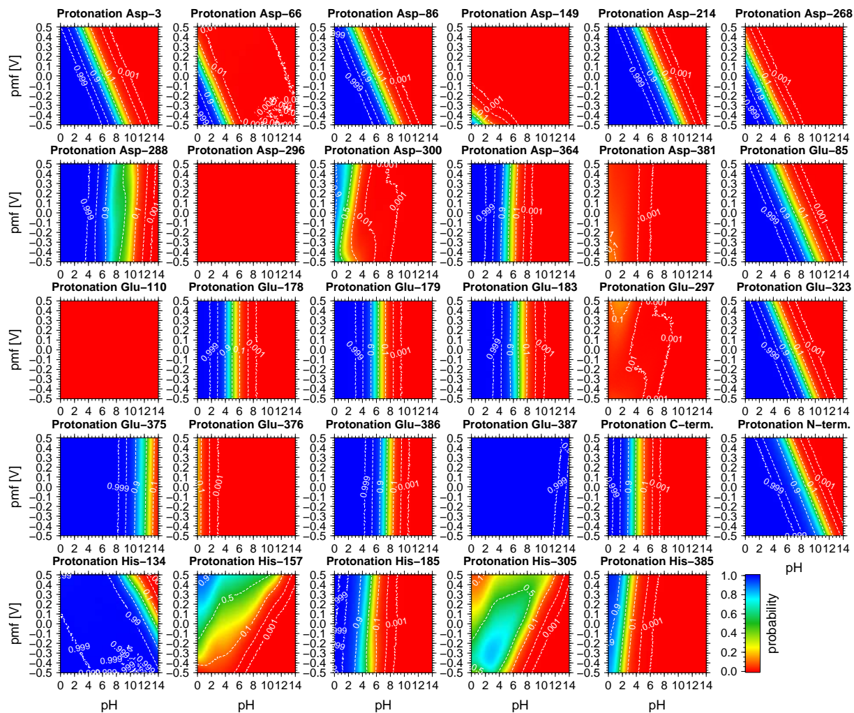
Figure S13: Titration curves \text{pH} - \Delta\text{pH} + \Delta\psi . Protonation probability as a function of the intracellular pH value and a pmf consisting of a transmembrane pH difference and an electric transmembrane potential. The ratio of the pH difference to the electric transmembrane potential is given by \frac{\Delta\psi}{\Delta\text{pH}} = 2 . The sites are indicated by the labels above the curves. The protonation probability is color coded (see color bar) and indicated by isocontours. Protonation of histidine residues refers to binding of a proton to one of the singly protonated charge-neutral tautomers to form the doubly protonated positively charged imidazolium form.
