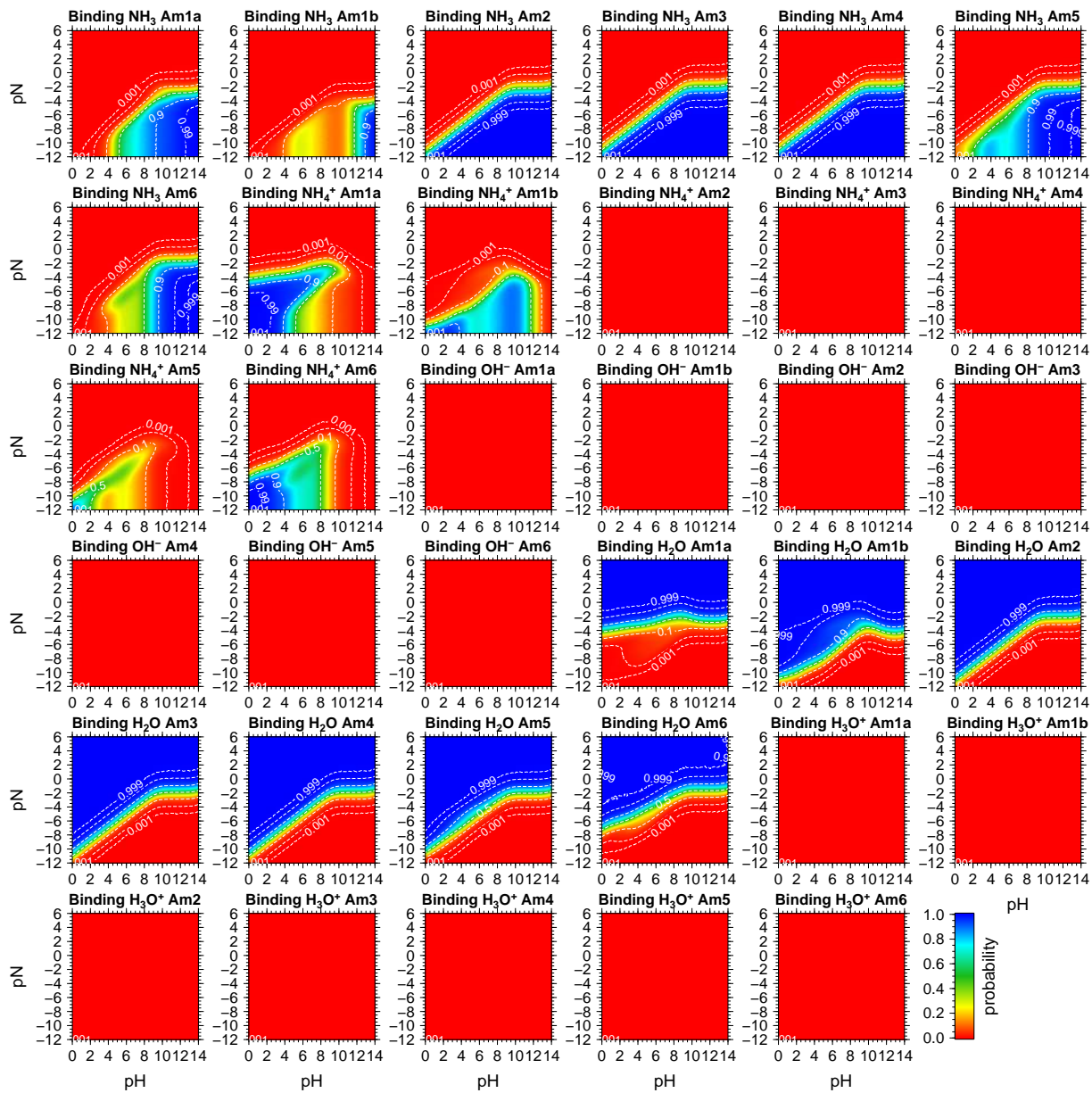
Figure S24: Titration curves intracellular pH - pN with pmf IV., (pN equal on both membrane sides, \Delta\text{pH}=1.0 , \Delta\psi = -120 mV). Continued from Fig. S23. See caption of Fig. S23 for explanation.
